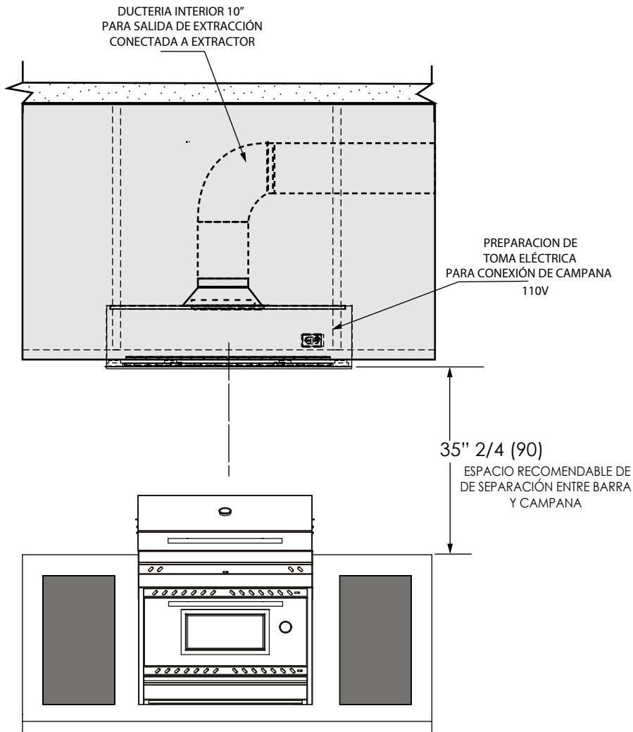
VISTA FRONTAL
